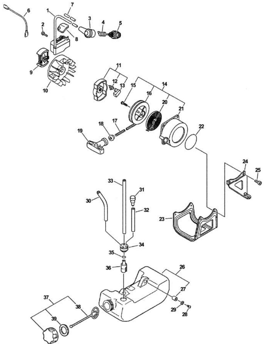
FIGURE 3 IGNITION, STARTER, CLUTCH, FUEL SYSTEM
