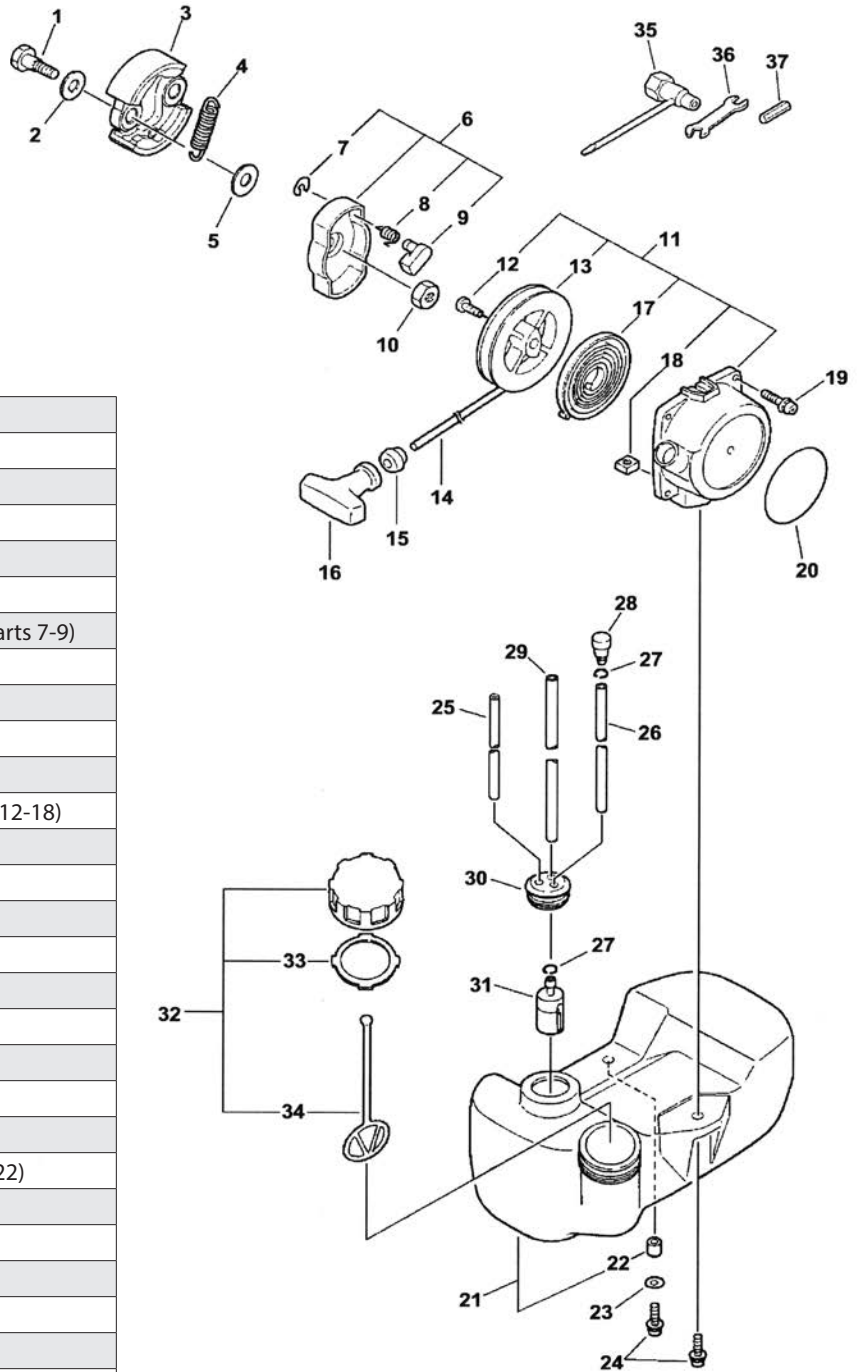
FIGURE 4 CLUTCH, STARTER, FUEL SYSTEM, TOOLS
