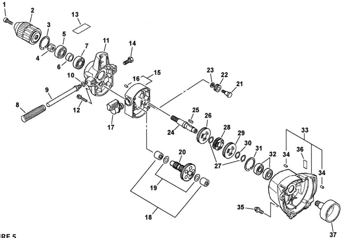
FIGURE 5 GEAR CASE, CLUTCH DRUM
