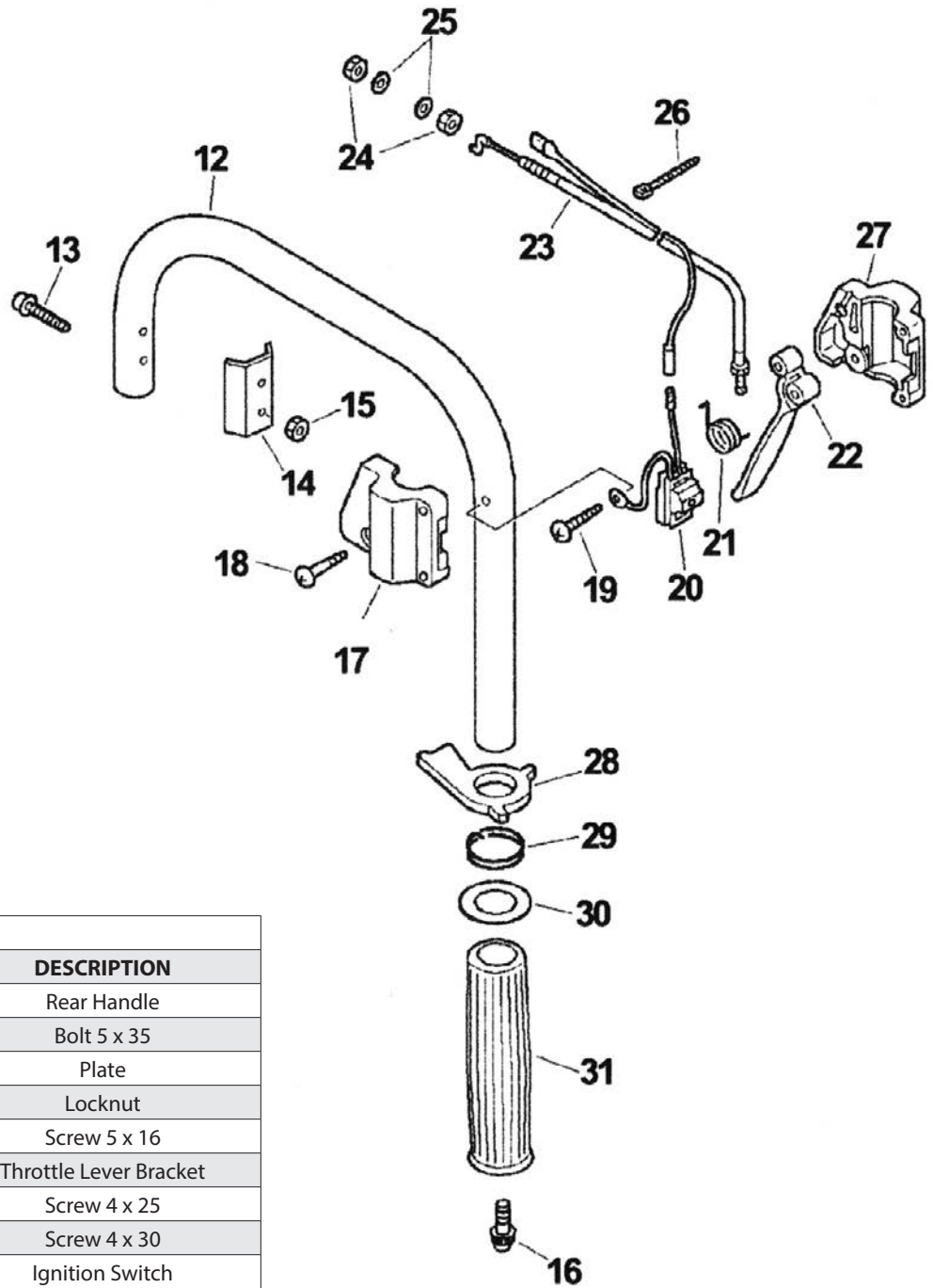
FIGURE 5 HANDLE, THROTTLE CONTROL
