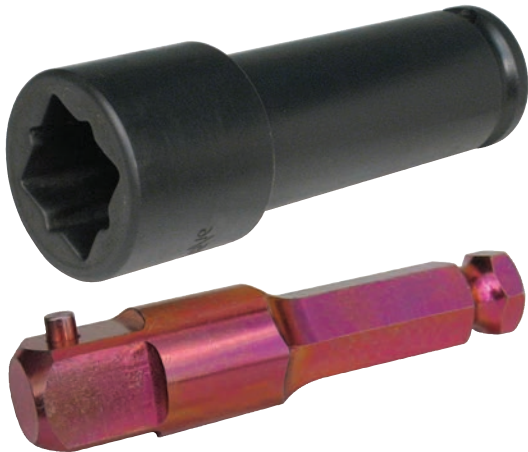
DOUBLE SQUARE IMPACT SOCKET 1/2" square drive, 5" long.
