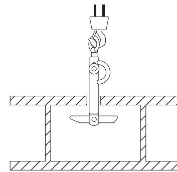
LIFTING CONFIGURATION
